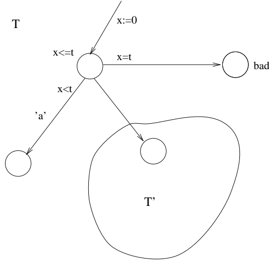
Fig. 5. Test Automata for \phi \text{Until}_{<t} a
