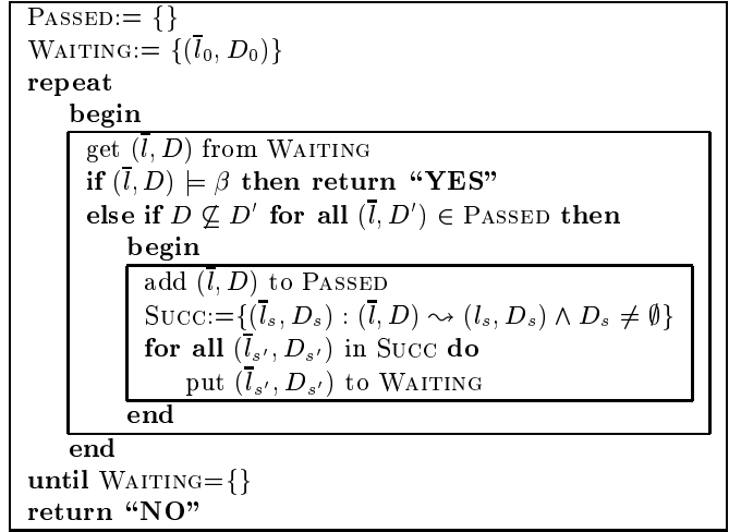
Fig. 6. An Algorithm for Symbolic Reachability Analysis.
