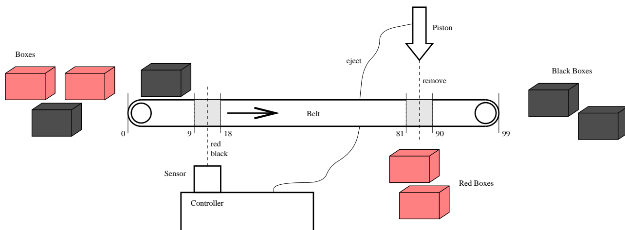
Fig. 7. The Box-Sorter Unit.
